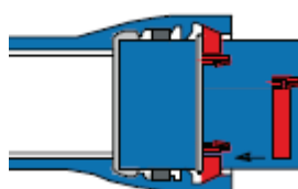
Lock Right segment
